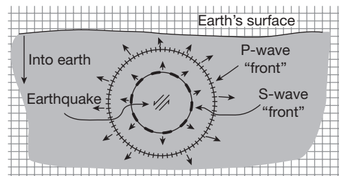
Figure 9.2 P (Primary) Waves and S (Secondary) Waves
